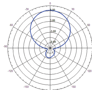
Total Gain - Azimuth
