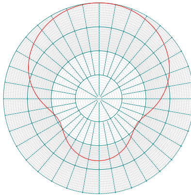
Right-hand circularly polarized linear azimuth plot.
